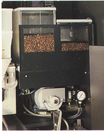
Dual hopper unit grinds and fresh brews both regular and decaf; single hopper grinds and fresh brews regular only.
